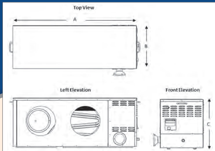
Figure: Dimensions locations (refer Table 2)
